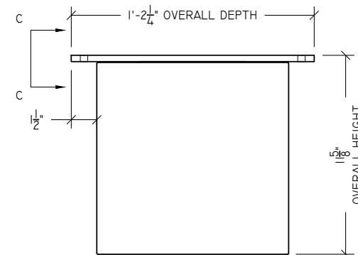
3 TOP MOUNT PLATE NOT TO SCALE
