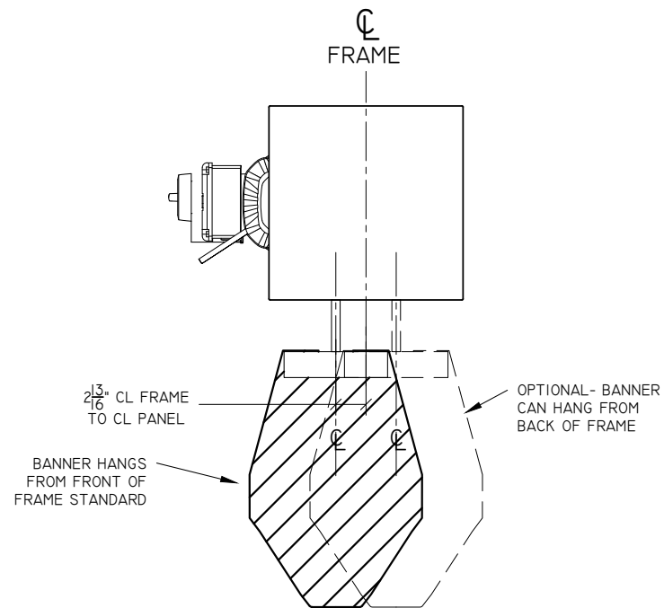
4 STAC OFFSET NOT TO SCALE
