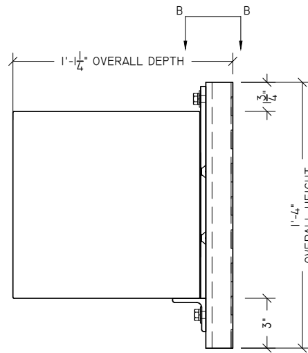
2 REAR MOUNT STRUT NOT TO SCALE
